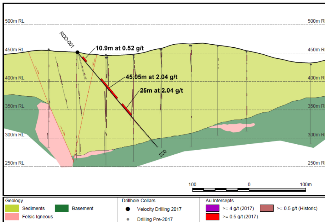
Figure 2: Section showing historical drill holes and Velocity’s drill hole number RDD-001. Intersections greater than 0.5 g/t gold are shown on historical drill holes. Intersections of gold mineralization are labelled.
