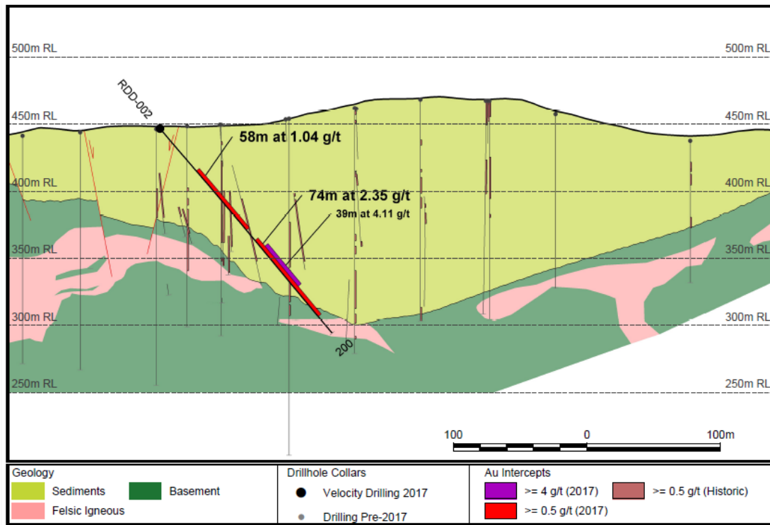
Figure 1: Section showing historical drill holes and Velocity’s drill hole number RDD-002. Intersections greater than 0.5 g/t gold are shown on historical drill holes. Intersections of gold mineralization are labelled.
