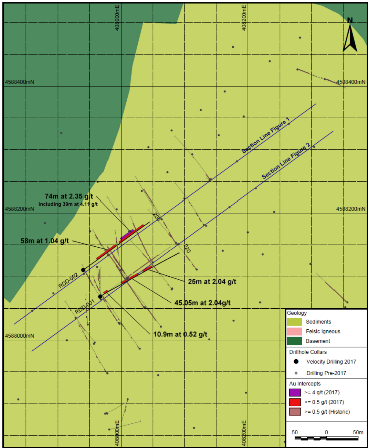
Figure 3: Map showing the location of historical drill holes and Velocity drill holes discussed in this news release. Historical drill holes are dominantly drilled vertically or angled toward the northwest. Velocity drill holes are angled toward the northeast. The locations of sections (Figure 1 and Figure 2) are also shown.
