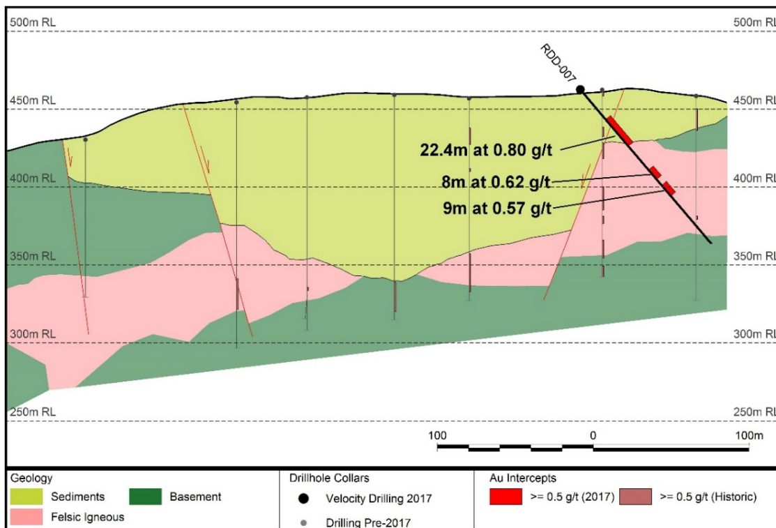
Figure 2: Drill Intersect from Velocity Hole RDD-007 at Rozino.
