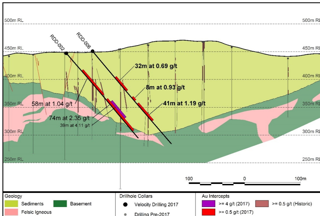
Figure 1: Drill Intersect from Velocity Hole RDD-006 at Rozino. Results for RDD-002 were released previously.
