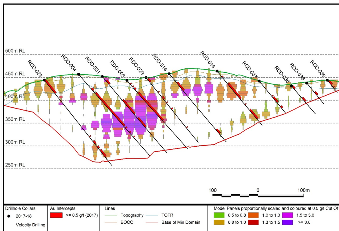
Figure 2. Representative section of resource estimate scaled and coloured by proportion above 0.5g/t gold cut off grade
