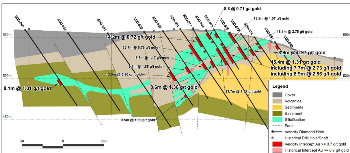
Figure 2: Cross Section X at Sedefche Gold Project showing results for drill holes ODD-071, -72, and -073.
