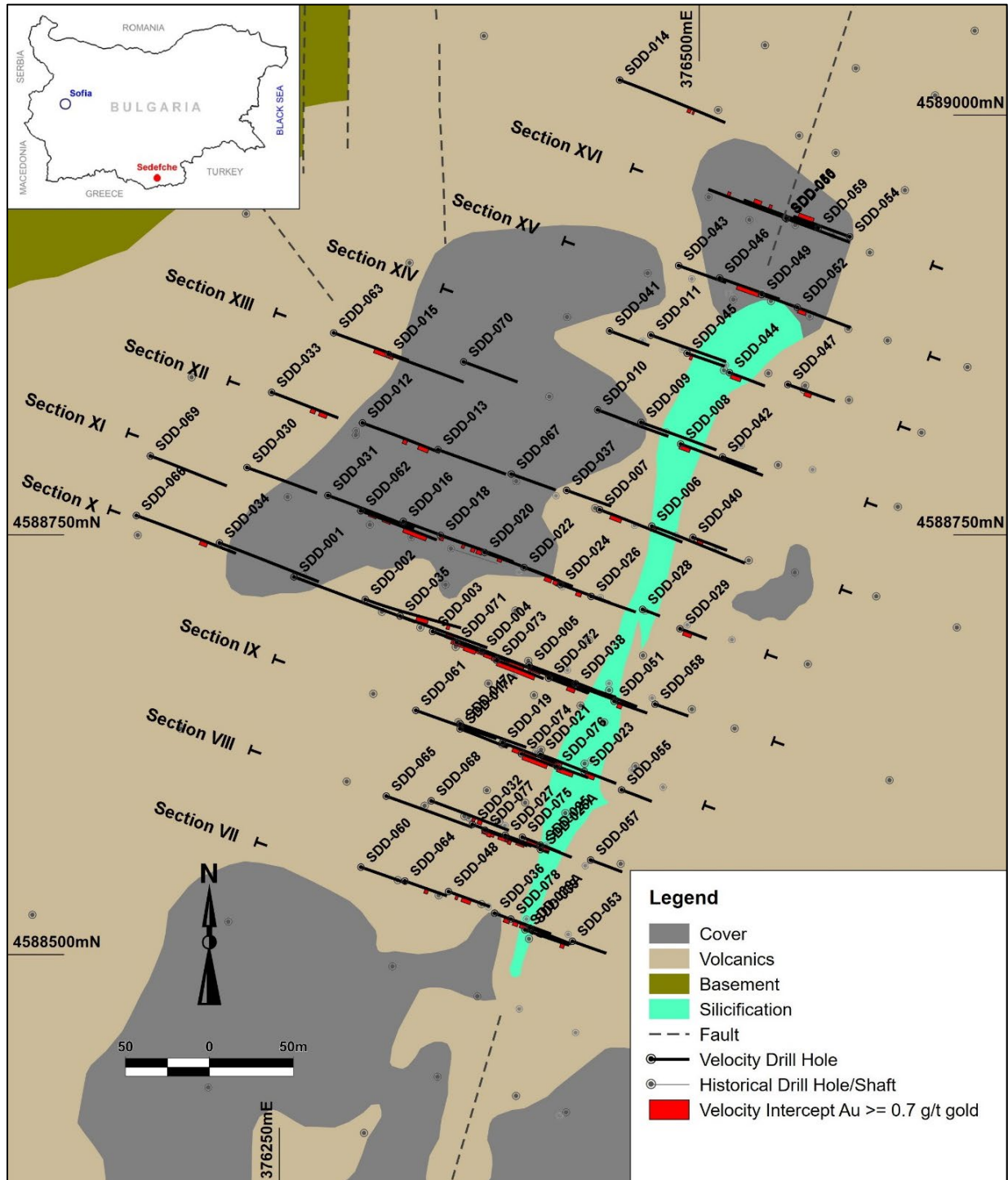
Figure 3: Map of the Sedefche Gold Project, showing Phase 1 drill traces. Drill hole locations are displayed on a geological map including positions of historic drill collars (section locations included for Figures 1 & 2).
