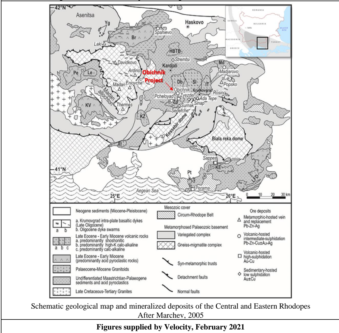
Figure 4: Regional geological setting
