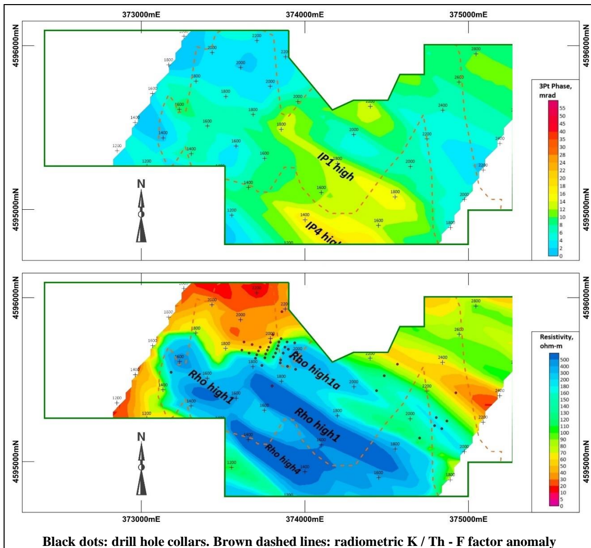
Figures supplied by Velocity in February 2021 Figure 13: Induced Polarization/Resistivity survey
